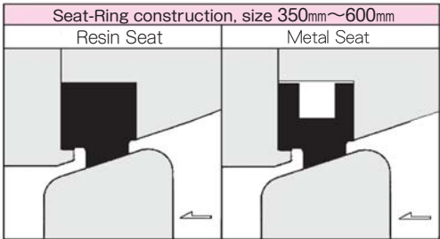
Vacuum Spec. (16BV)
