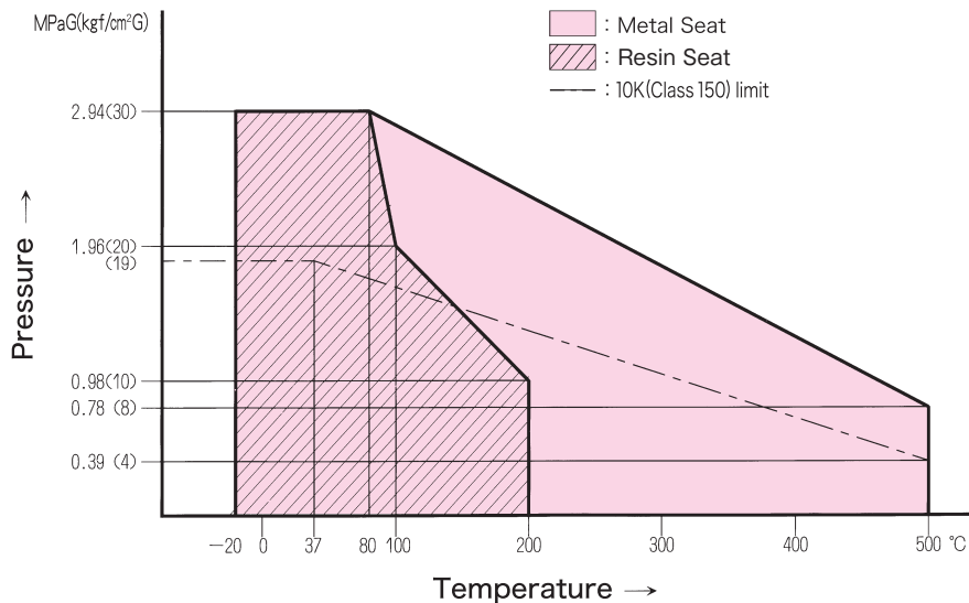
Applicable Pressure-Temperature Range
