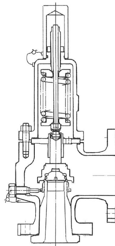
FIG.2 Style JNO closed bonnet
