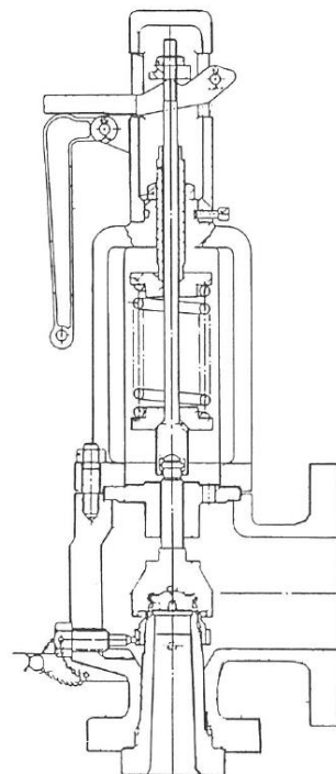
FIG.3 Style JNO-H open bonnet
