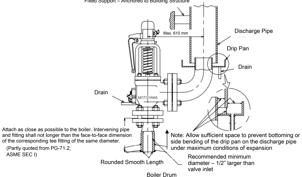
Fixed Support – Anchored to Building Structure
