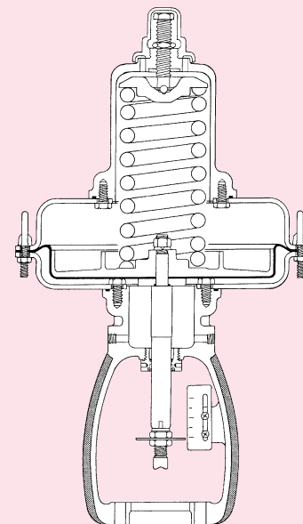
Reverse Action (RA) (Air-to stem up)
